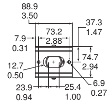
LTC 9219/01 Feed-through J-Mount
